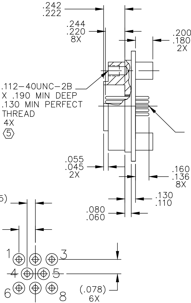
INSERT ARRANGEMENT
